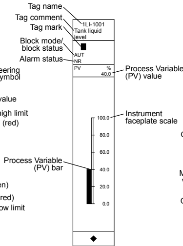
Figure PVI Input Indicator Block
