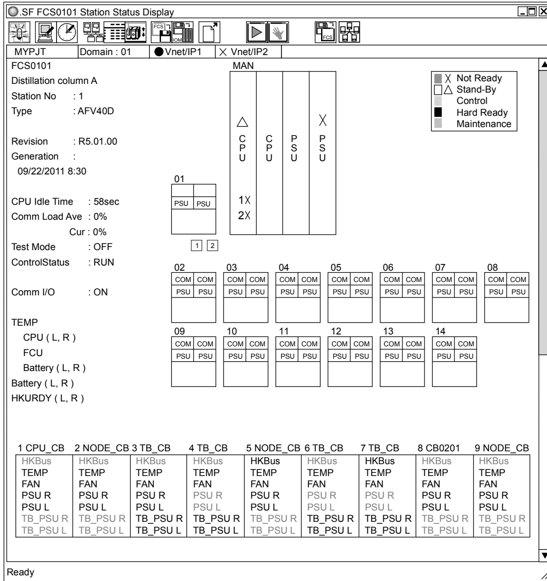
Figure FFCS-V Status Display View (With Cabinet)
