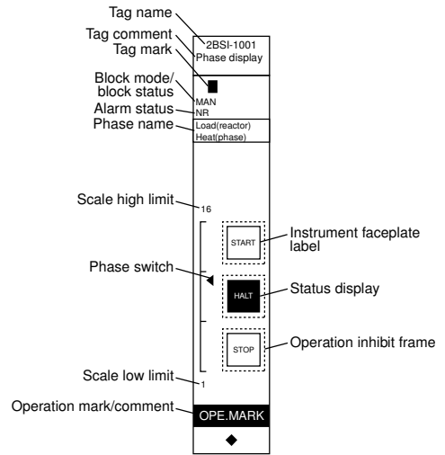
Figure BSI Batch Status Indicator Block
