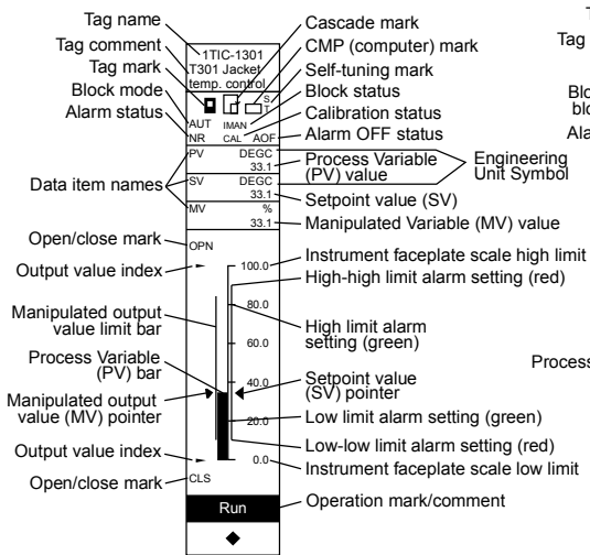
Figure PID Controller Block
