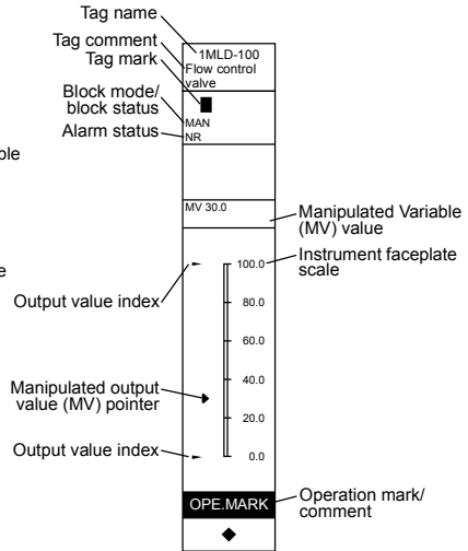
Figure MLD Manual Loader Block
